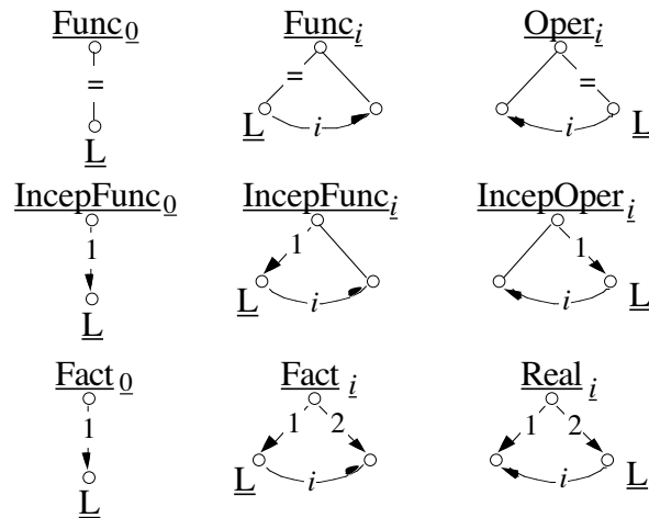
Figure 7: Derivation structures of some lexical functions ( L is the base word)
