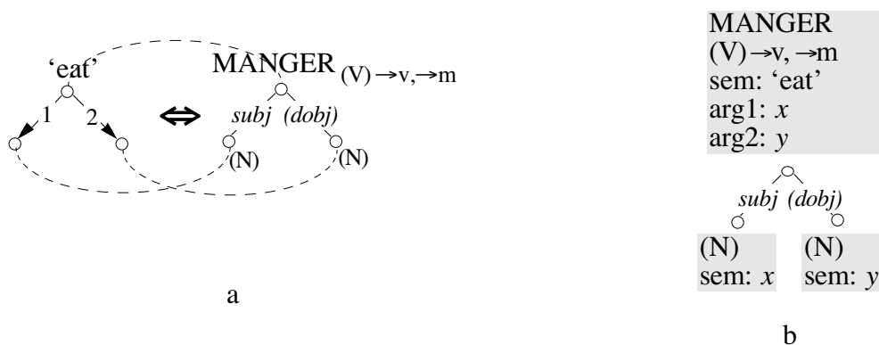
Figure 1: Two representations for the rule for MANGER 'eat'
