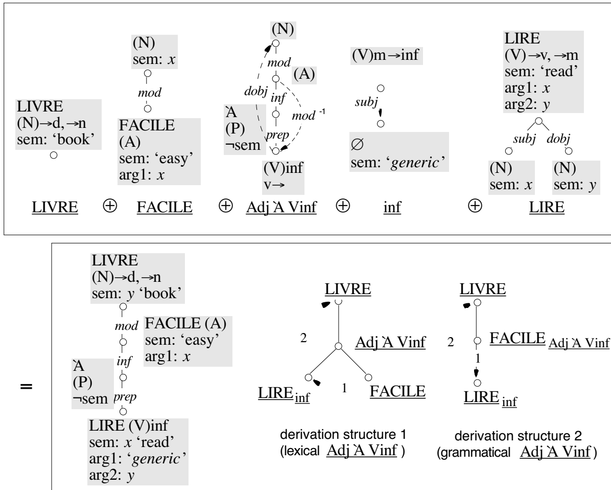
Figure 8: Derivation of un livre facile à lire ‘a book easy to read’
