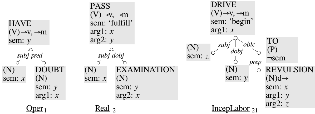
Figure 6: Collocates HAVE , PASS , and DRIVE
