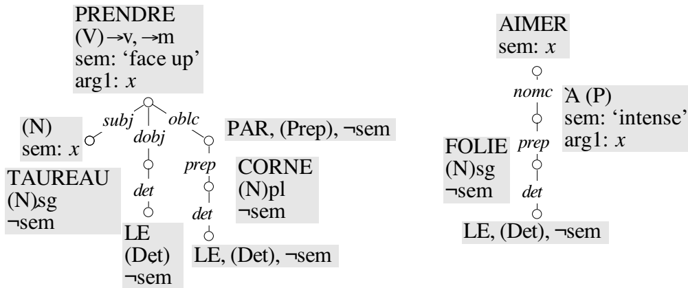
Figure 5: The idiom PRENDRE LE TAUREAU PAR LES CORNES ‘take the bull by the horns’ = ‘face up’ and the collocate A LA FOLIE ‘to the madness’
