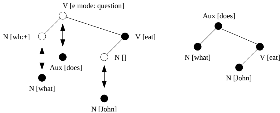
Figure 5: Trees for eats with wh -movement and other trees (left); derived tree (right).
