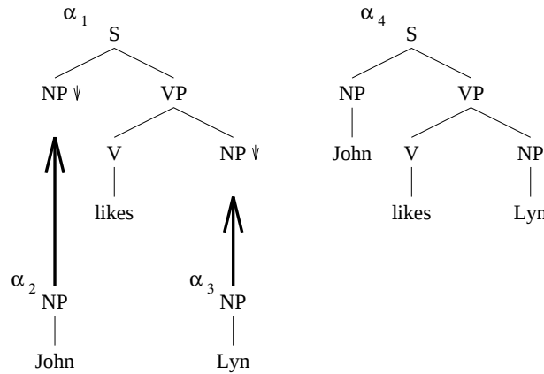
Figure 2: Substitution of arguments into initial tree of likes
