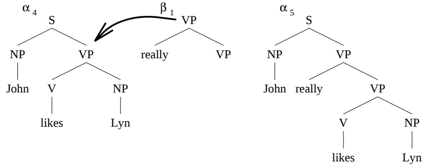
Figure 3: Adjunction of really into initial tree
