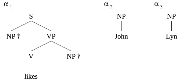
Figure 1: A sample Tree Adjoining Grammar
