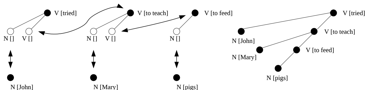
Figure 7: Trees for German nested dependencies
