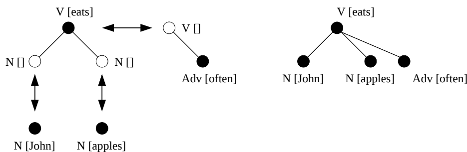
Figure 4: Some elementary tree (left) with attachments; final derived tree (right). Double-headed arrows show attachments.
