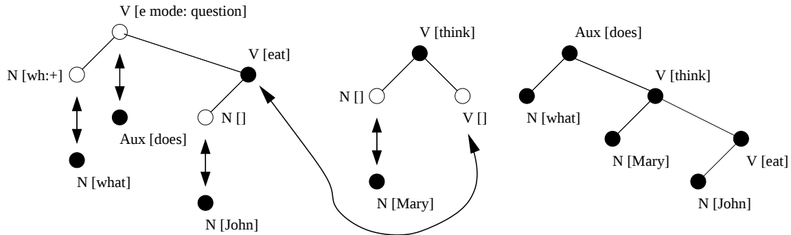
Figure 6: Tree for eats with long-distance wh -movement (left); derived tree (right).
